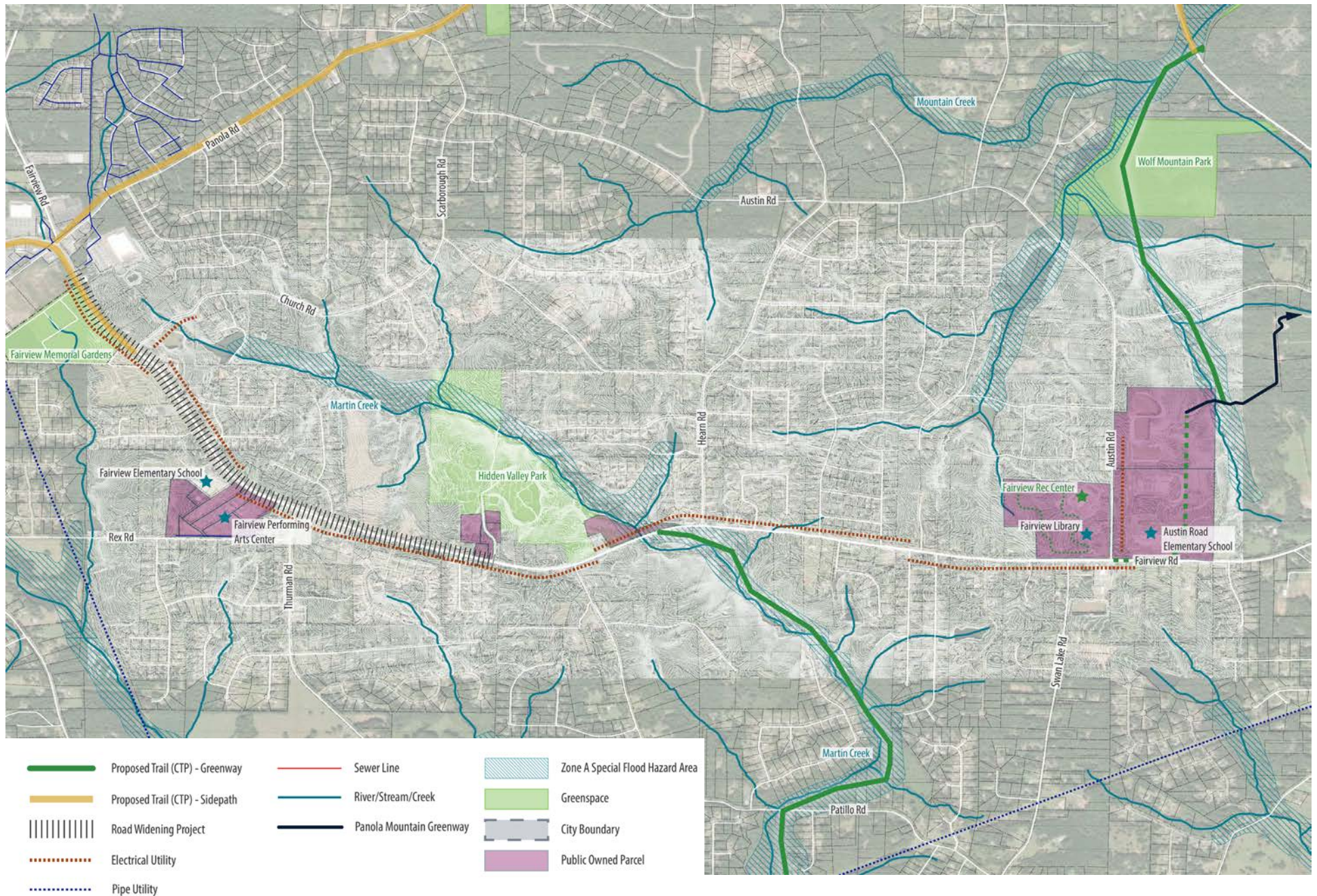
Figure 4.7. Fairview Model Mile Existing Conditions
