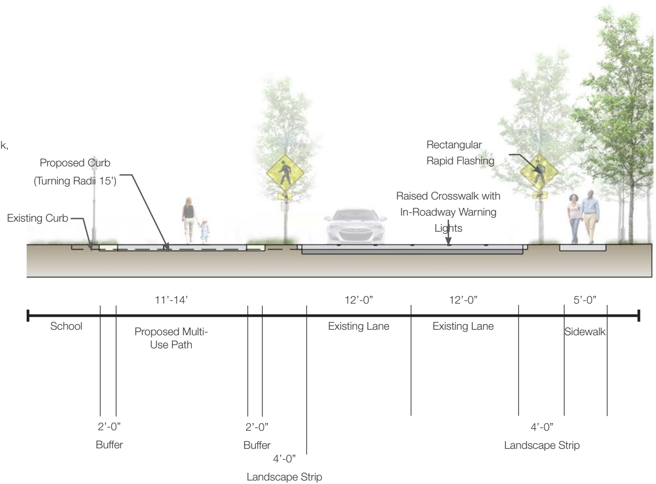
Figure 4.14. Proposed Traffic Calming at School Section
